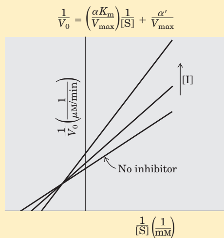
FIGURE 3 Mixed inhibition.
