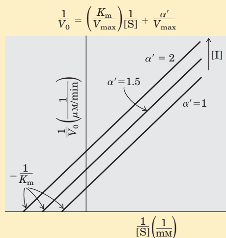
FIGURE 2 Uncompetitive inhibition.
